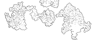
PB1
